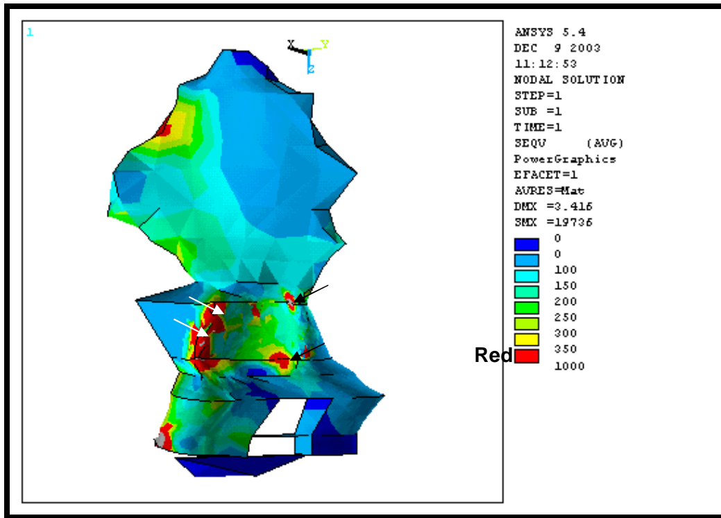
Fig 7: Von Mises stress distribution on the lateral surface of the hip bone in a 70 kg body by using ANSYS program for FEA.
