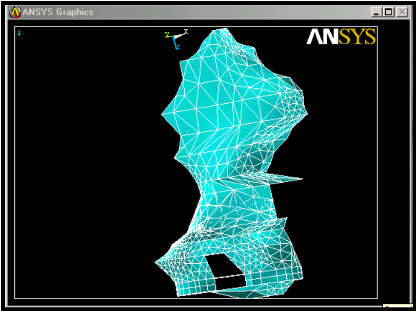
Fig.3 computer screen after the model have been meshed
