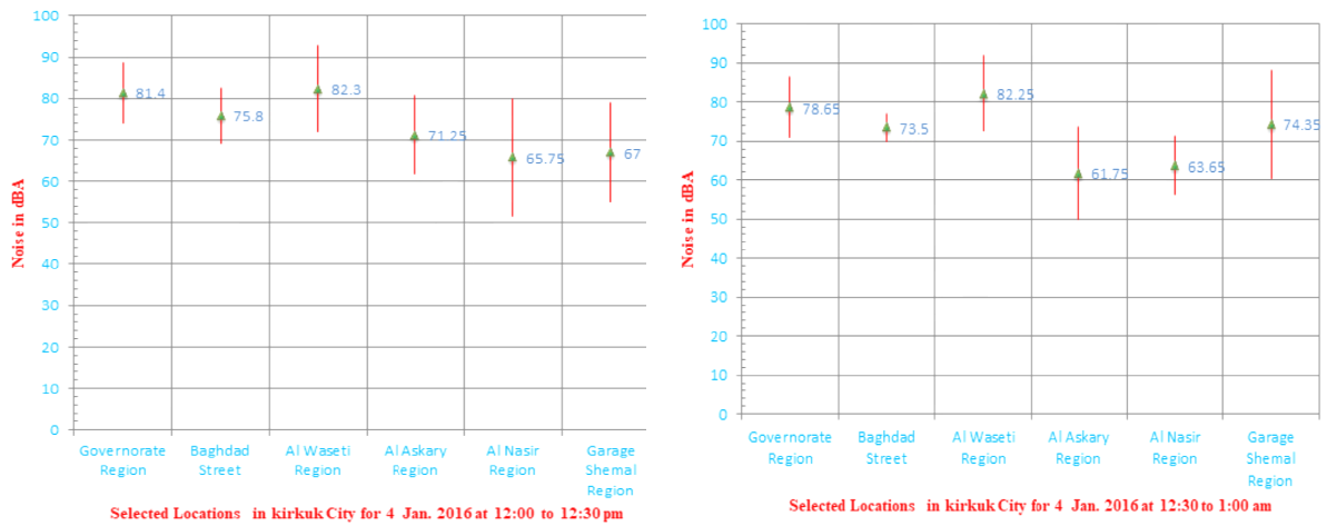
Fig. 11. Max , Min and Average Hourly Noise Distribution for the traffic flow 4 Jan. 2015 Kirkuk City.
