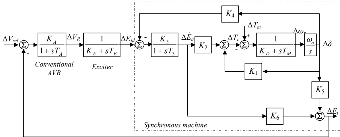
Fig. 8. Detailed Block Diagram of the Linearized Excitation System.
