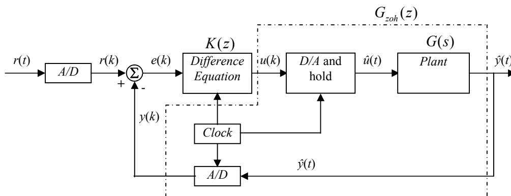
Fig. 2. Closed-loop Control System.
