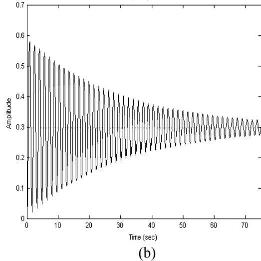
Fig. 10. Output Response of \Delta E_t due to a 0.3 pu Step Increase in \Delta V_{ref} , (a) K_A = 10 , (b) K_A = 50 .
