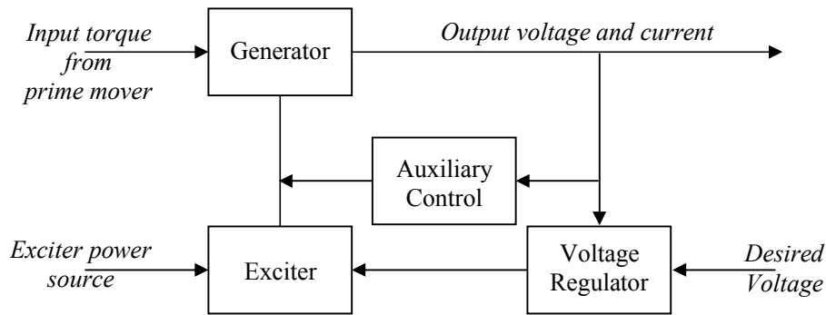
Fig. 6. Typical Arrangement of Excitation Components.
