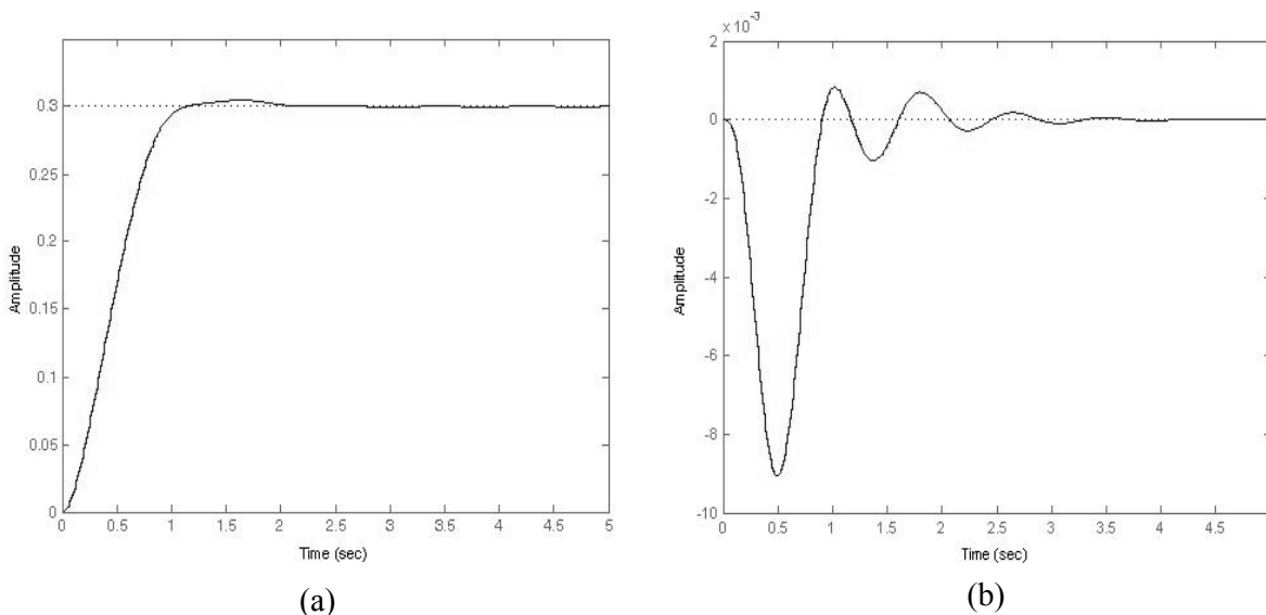
Fig.12. Output Response of the Excitation Control System with DAVR due to a \Delta V_{ref} = 0.3 pu , (a) \Delta E_t , (b) \Delta \omega_r .
