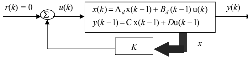
Fig. 4. Quadratic Optimal Control System.
