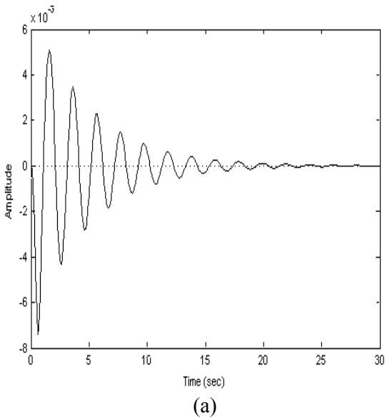
Fig. 11. Output Response of \Delta\omega_r due to a 0.3 pu Step Increase in \Delta V_{ref} , (a) K_A = 30 , (b) K_A = 50 .
