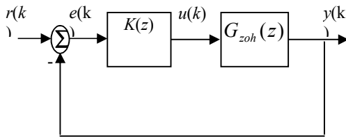
Fig. 3. Closed-Loop Digital Control System.
