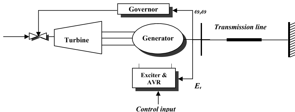
Fig. 7. Power System Configuration.
