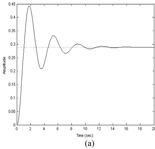
Fig. 10. Output Response of \Delta E_t due to a 0.3 pu Step Increase in \Delta V_{ref} , (a) K_A = 10 , (b) K_A = 50 .
