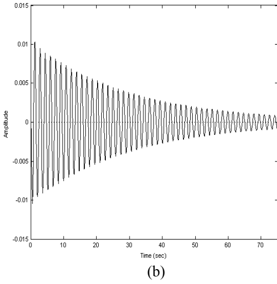
Fig. 11. Output Response of \Delta\omega_r due to a 0.3 pu Step Increase in \Delta V_{ref} , (a) K_A = 30 , (b) K_A = 50 .
