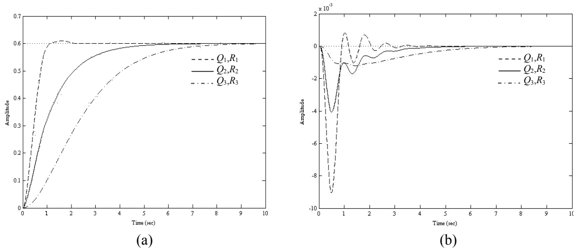
Fig.14. Output Response of the Excitation Control System ( \Delta E_t ) due to a \Delta V_{ref} = 0.6 pu with Different DAVRs, (a) \Delta E_t , (b) \Delta \omega_r .
