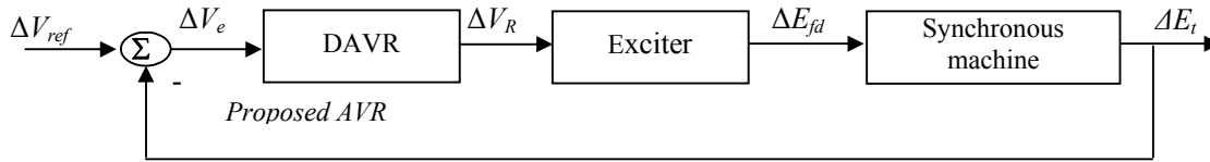
Fig. 9. Block Diagram of the linearized Excitation Control System with the Proposed Digital AVR (DAVR).
