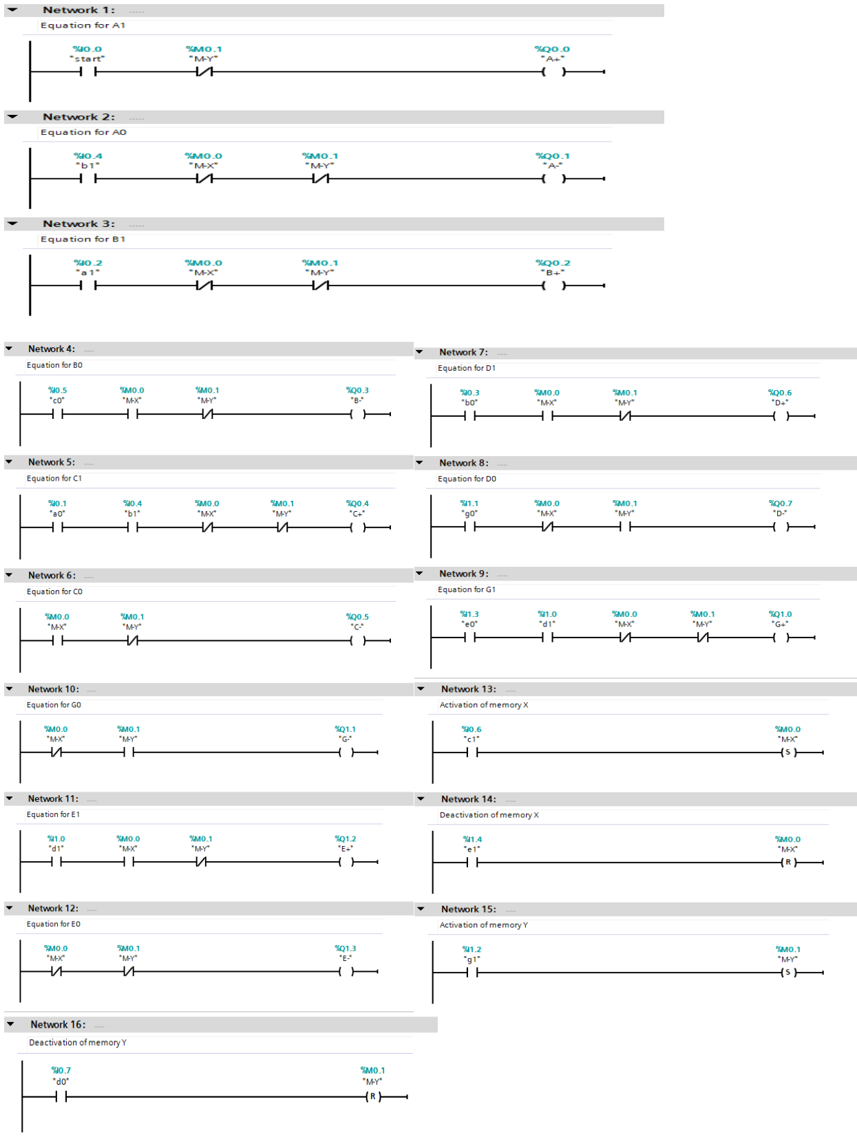
Fig. 9. PLC program in Ladder language.
