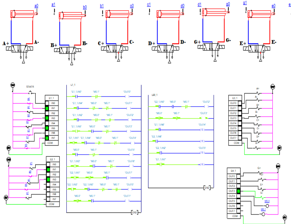
Fig. 8. Ladder implementation.
